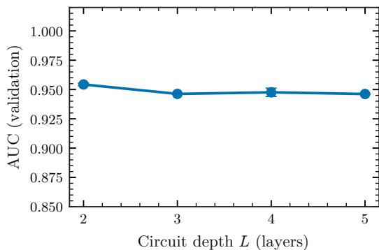
Figure 5. VQC hyperparameter sweep -- real parameter-shift-rule training results
