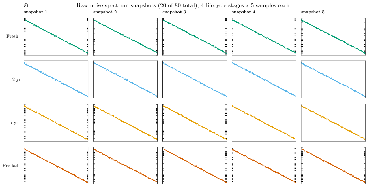
Figure 9. Raw-spectrum small-multiples gallery and rigorous statistical hypothesis testing
