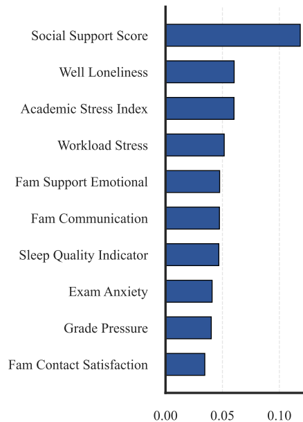
(c) CatBoost
