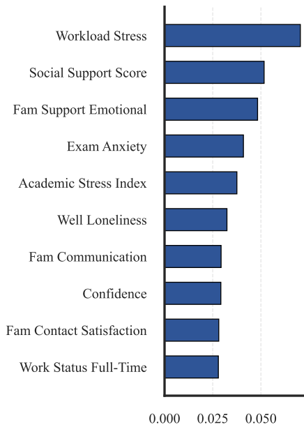
(b) XGBoost
