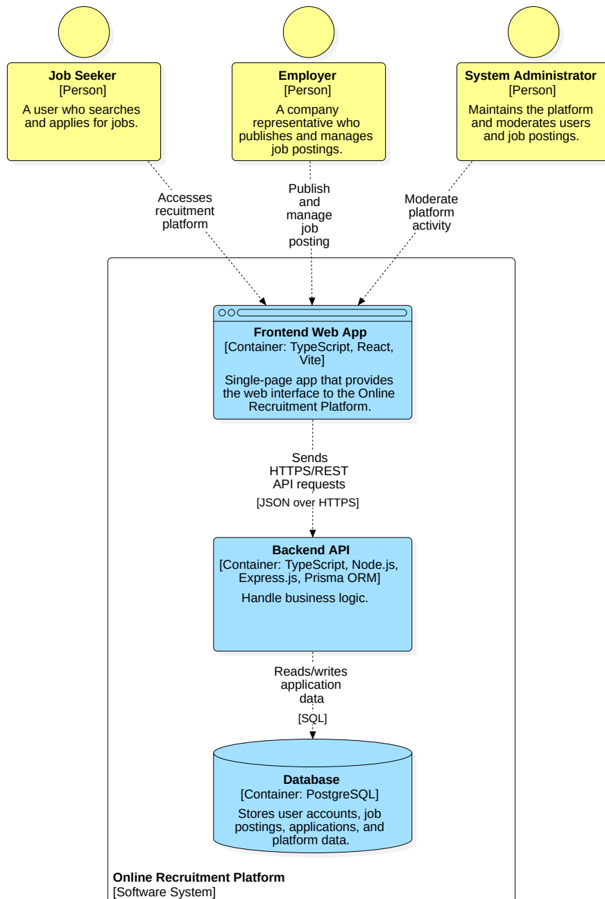
Figure 3.2: Container Diagram.
