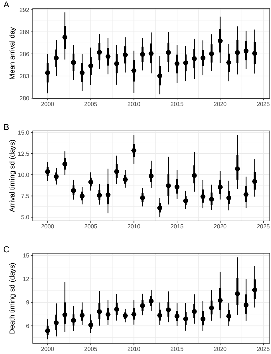
Figure 5: Posterior distributions of timing, entry_spread, and exit_spread. Points and error bars show the posterior median and the 66% and 95% credible intervals.
