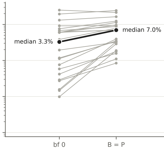
NVENC, QP 28 (22/23 sequences up)
