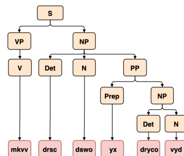
Figure 1: Parse Tree of a Sentence of Source Language
