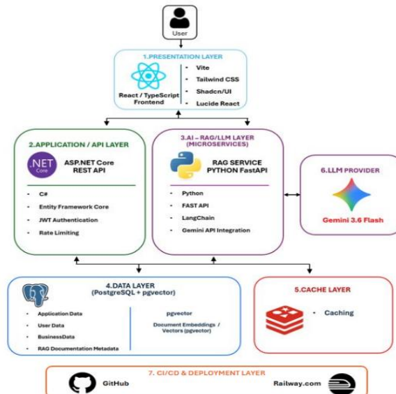
Figure 1.1 shows the overall technology architecture of the GT Companion platform.
