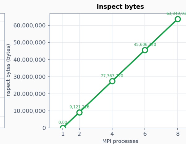
Triangle Counting scalability — Wikipedia talk (temporal)
