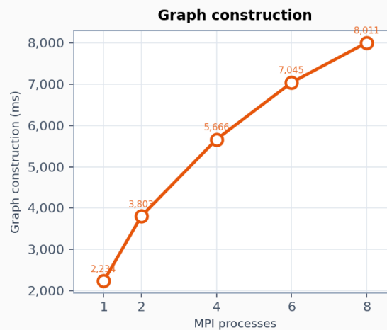
Triangle Counting scalability — Web graph — Google
