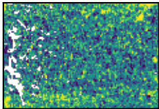
(b) Al-OH, 2.2 \mu\text{m}
