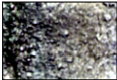
(a) VNIR colour
