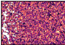
(c) Mg-OH, 2.3 \mu\text{m}
