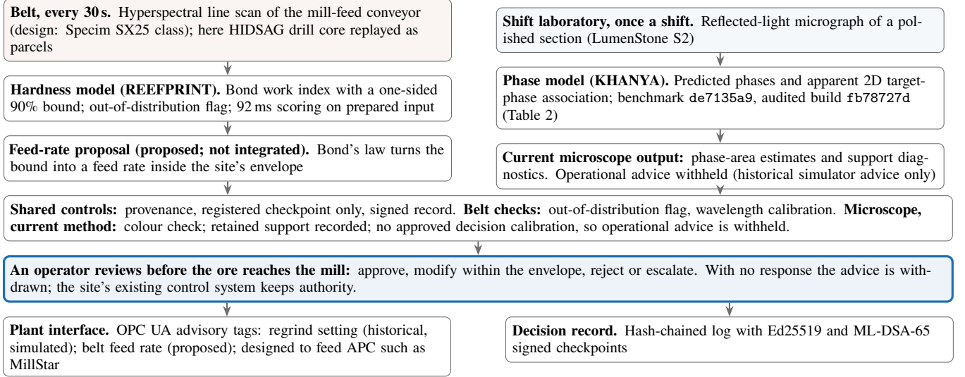
Figure 1: System architecture: two measurement cadences, one operator workflow. The belt and microscope branches produce model estimates at different cadences; the microscope gives predicted phase labels and apparent 2D target-phase association, and independent laboratory measurements provide the reference evidence. Shared provenance and operator controls are supplemented by branch-specific checks. Built: the models, applications and signed record (on replayed public data). Simulated (historical): the plant and regrind interface. Proposed: the belt sensor and feed-rate path. Microscope advice is withheld in the current method.
