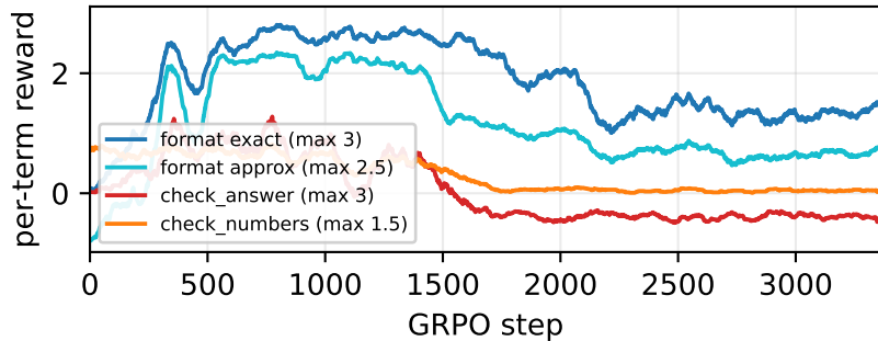
R0 ( K = 2, \beta = .08 ): collapse
