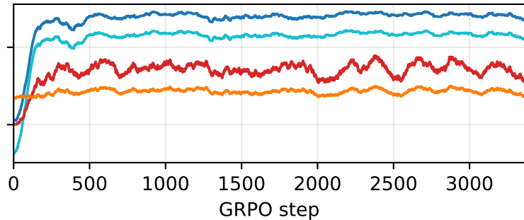
R3b ( K = 8, \beta = 0 ): stable
