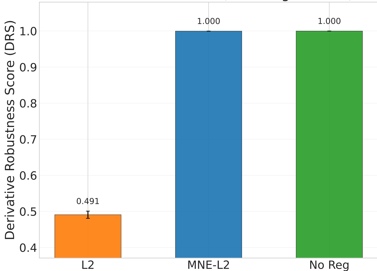
CIFAR100 VGG16: DRS (three regularizers)
