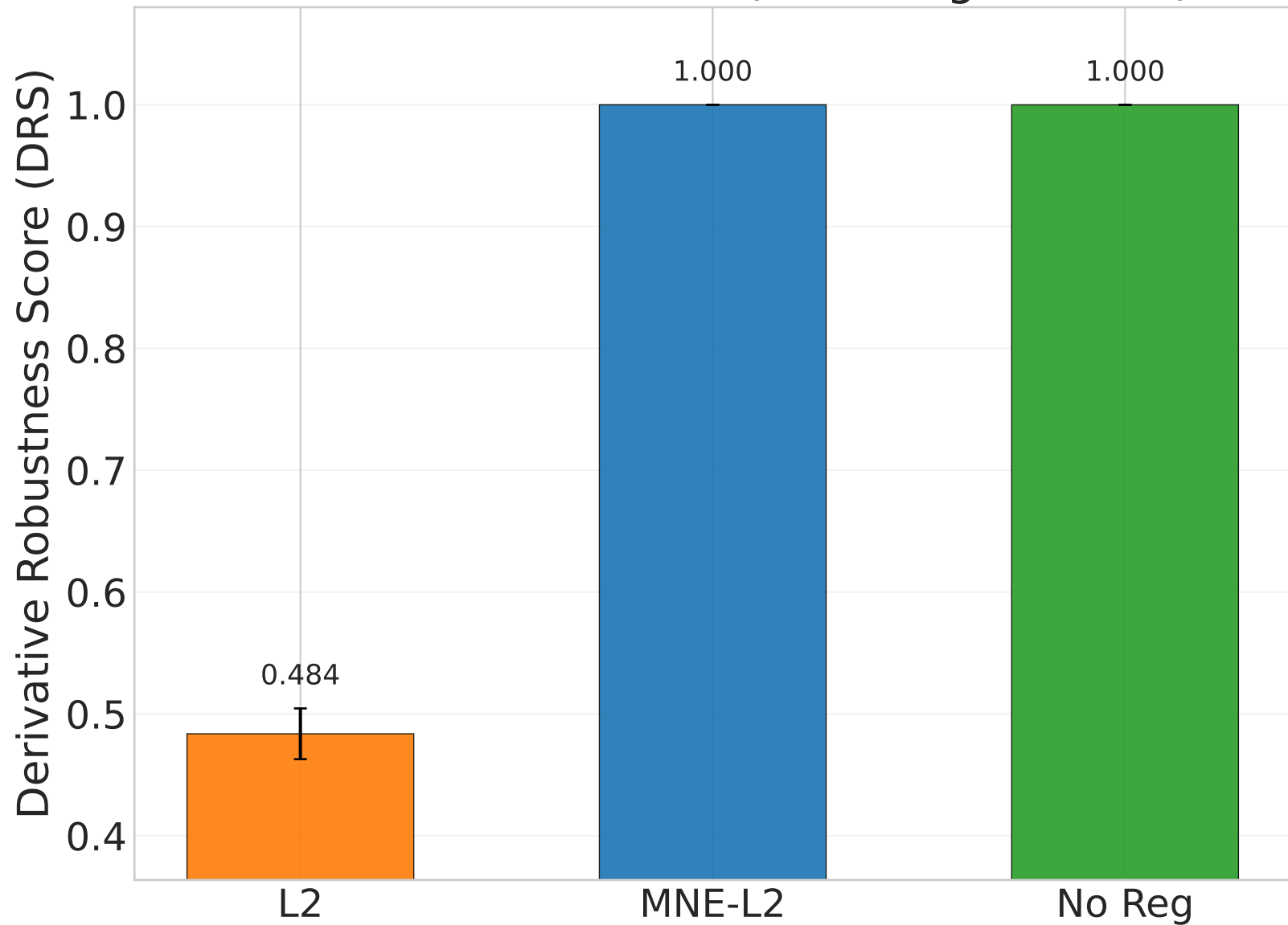
CIFAR10 VGG16: DRS (three regularizers)
