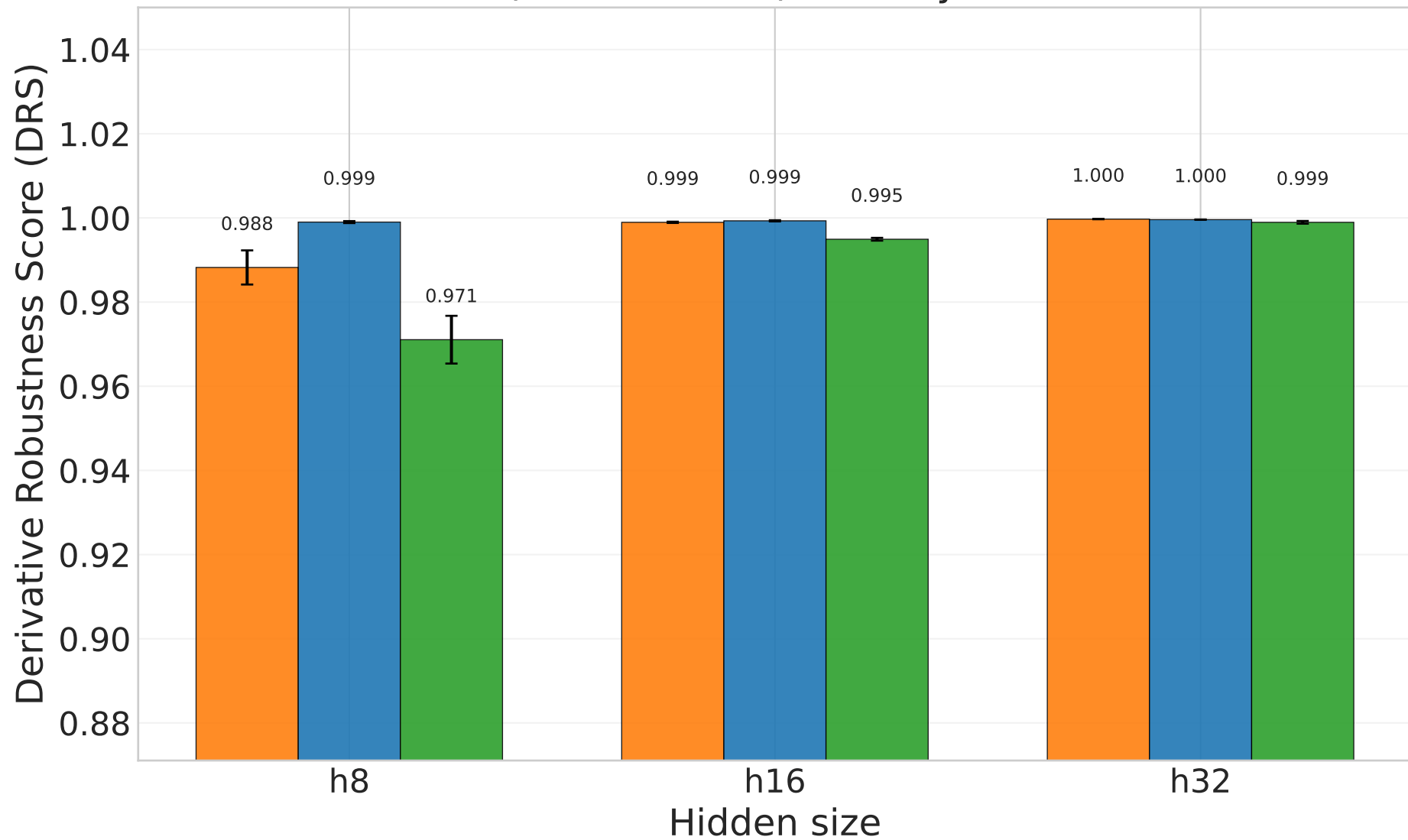
L2 MNE-L2 No Reg FC3rev (MNIST, 2h→h): DRS by hidden size
