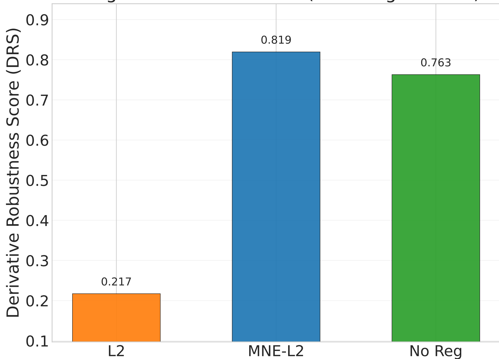
ImageNet ResNet18: DRS (three regularizers)
