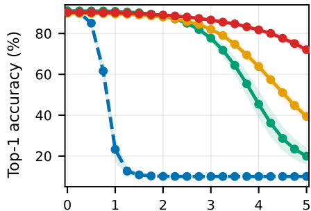
(a) CIFAR-10 VGG16
