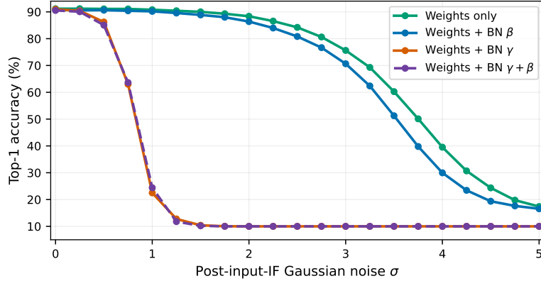
Figure 1: CIFAR-10 VGG16 L2 parameter-scope ablation at L = T = 16 . Gaussian noise is injected after the input IF. The training seed is fixed at 42 and each point uses one stored perturbation stream, so no uncertainty band is shown. Regularizing BN- \gamma , with or without BN- \beta , causes the early collapse.
