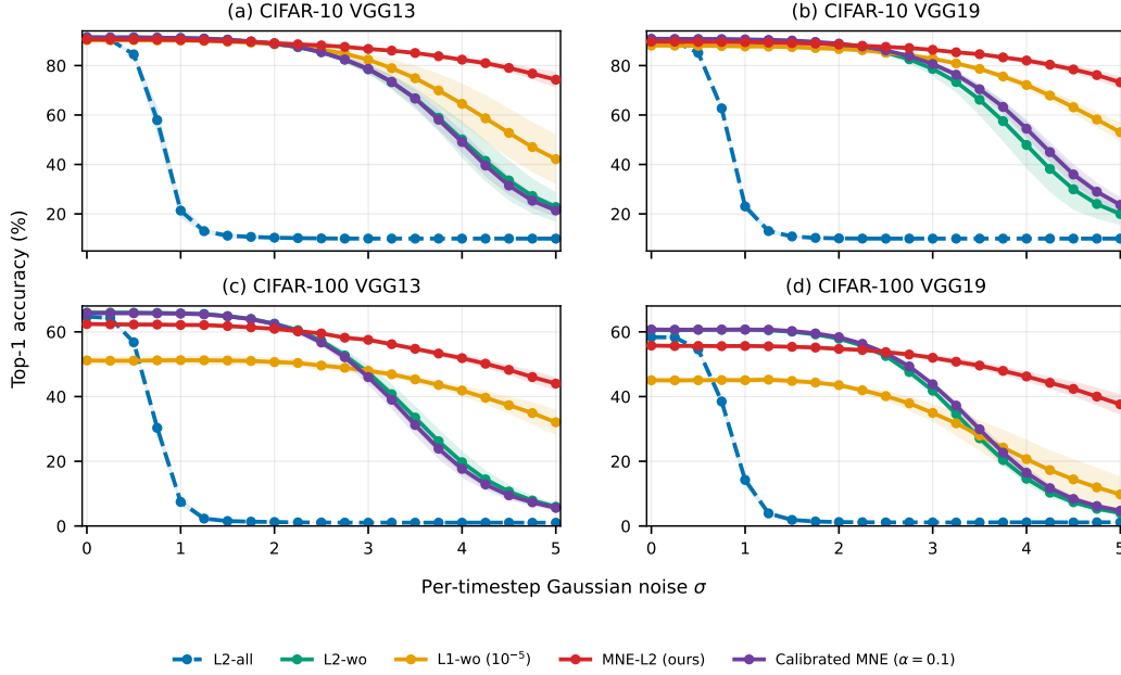
Figure 4: Depth-transfer robustness at L = T = 16 under Gaussian noise applied independently at each SNN timestep. Curves are five-seed means and bands show sample standard deviations. MNE-L2 is highlighted in red; Calibrated MNE is included only as an appendix control.
