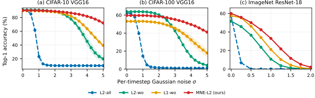
Figure 2: Per-timestep Gaussian-noise sweeps at L = T = 16 . (a,b) CIFAR VGG16 curves are five-seed means; bands show sample standard deviations across seeds 40–44. (c) ImageNet ResNet-18 uses one seed-42 checkpoint and therefore has no uncertainty band. MNE-L2 is highlighted in red and all data points use circular markers.
