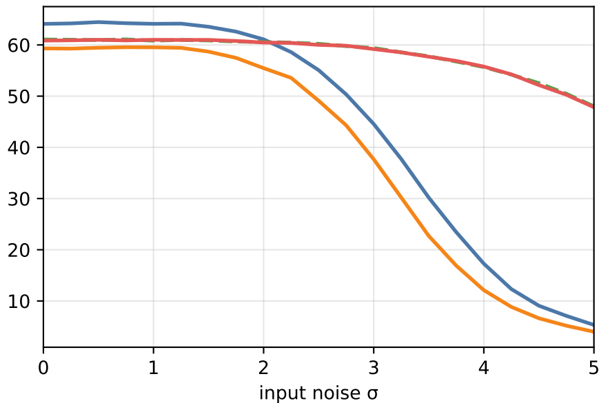
CIFAR-100 VGG16
