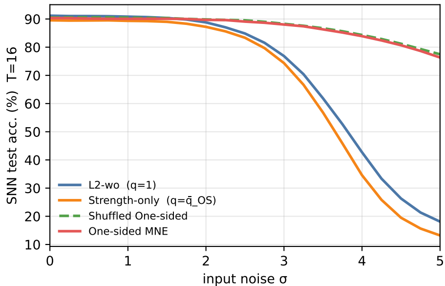
CIFAR-10 VGG16
