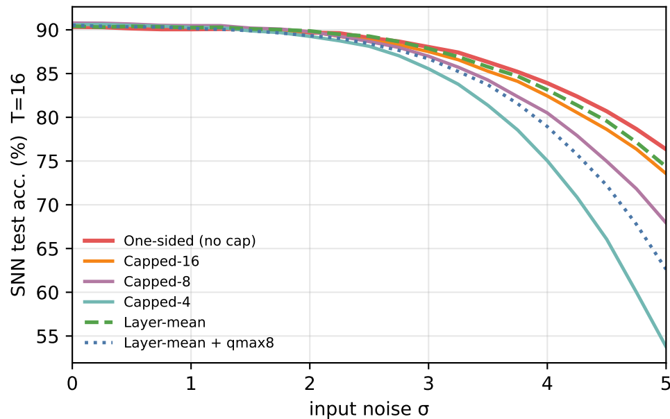
CIFAR-10 VGG16
