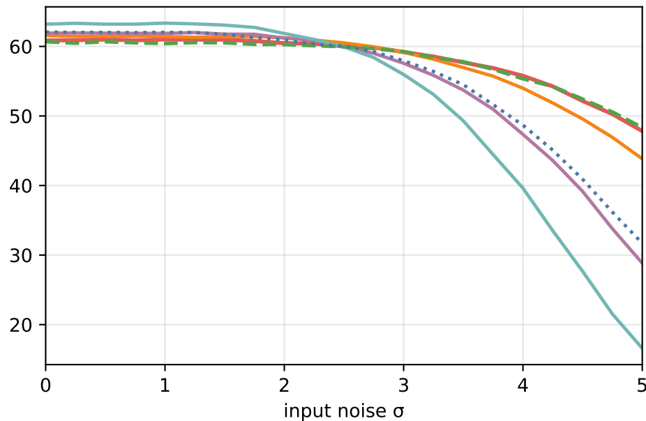
CIFAR-100 VGG16
