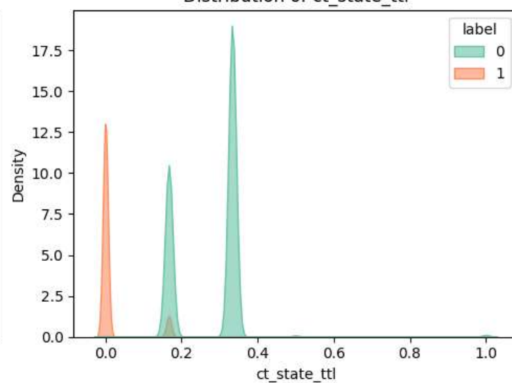
Distribution of ct_state_ttl
