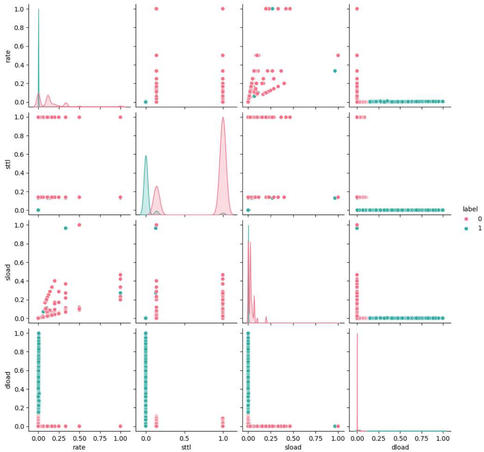
Pairplot of Top Features
