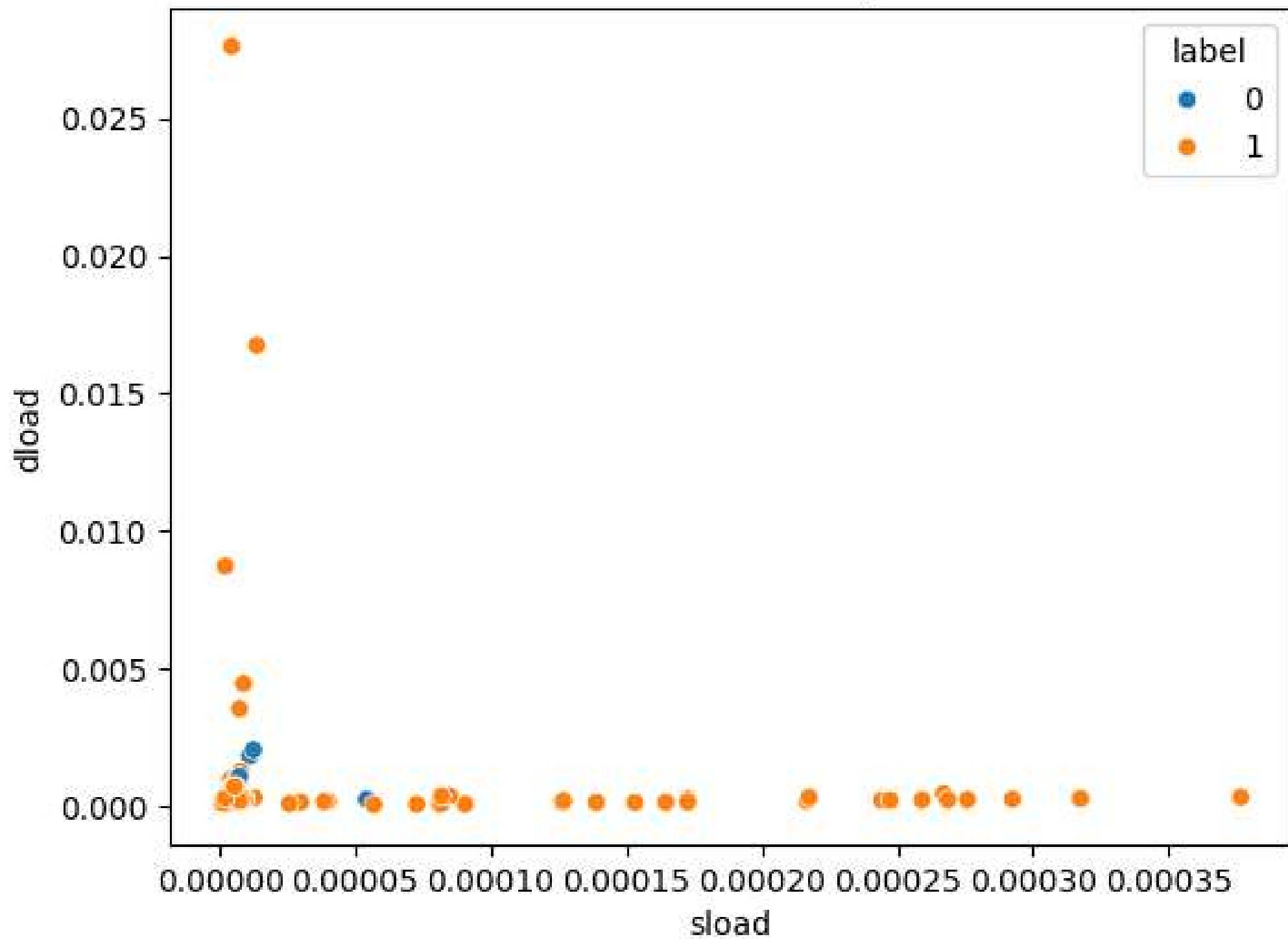
Misclassified Samples
