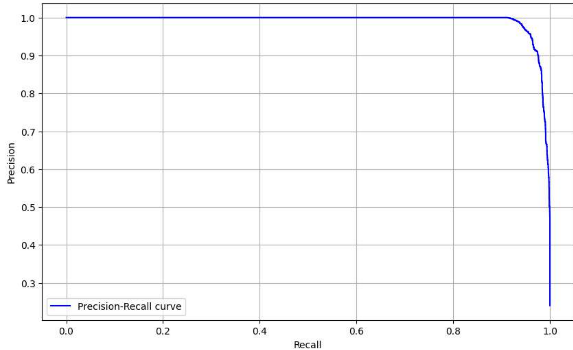
Precision-Recall Curve
