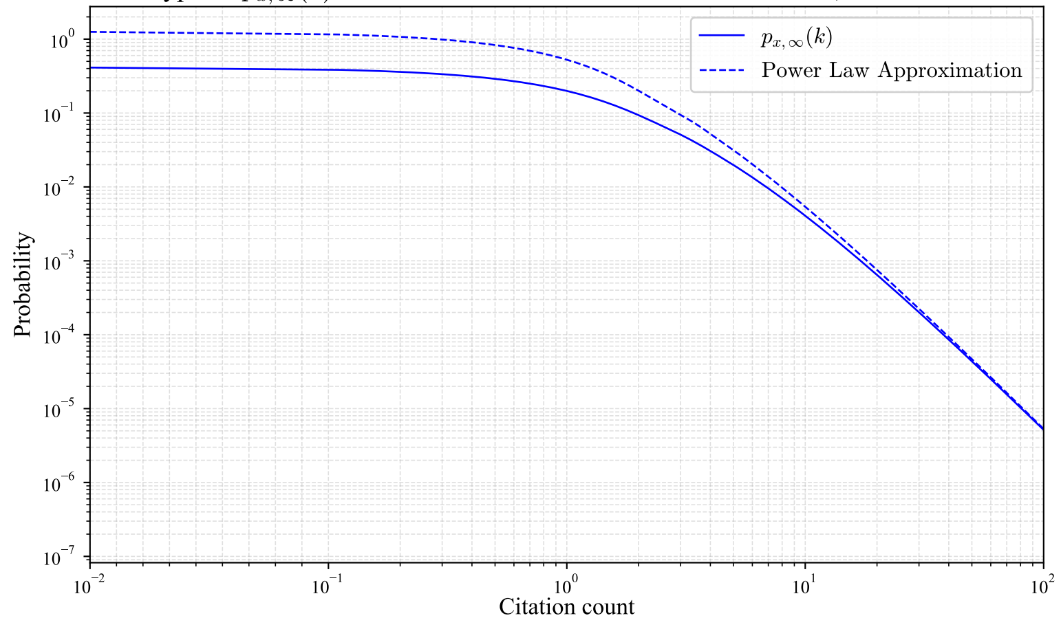
Type B: p_{x,\infty}(k) vs Power Law for Citation Distribution in 28,005 Network
