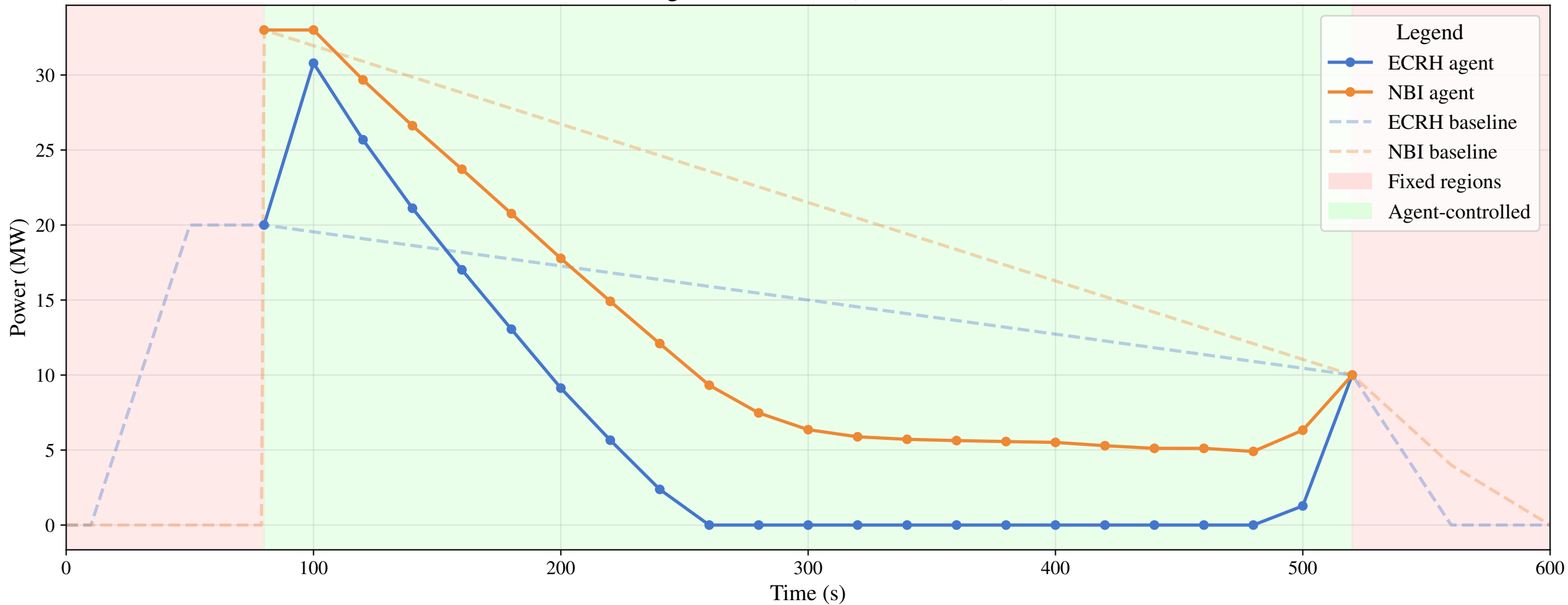
BC Agent vs. Baseline (reward=34.47)
