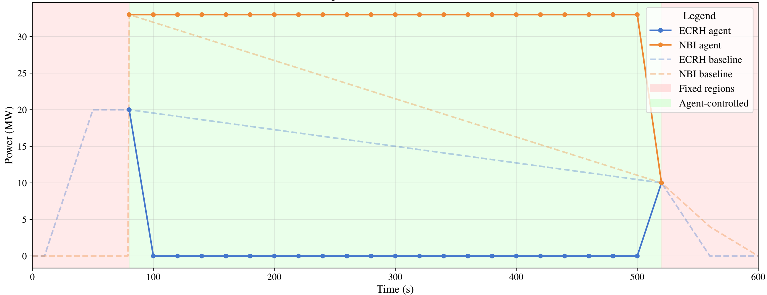
CQL Agent vs. Baseline (reward=12.91)
