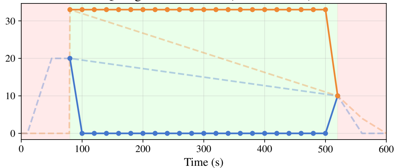
CQL Agent vs. Baseline (reward=12.91)
