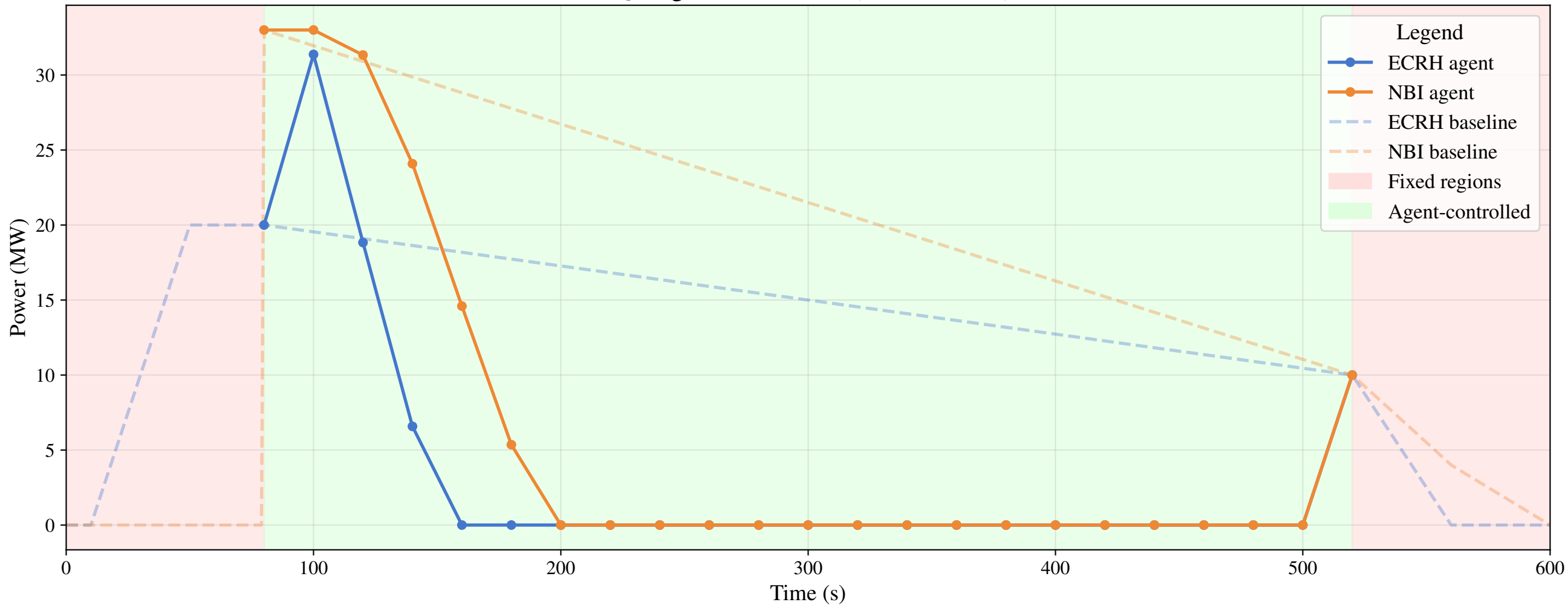
IQL Agent vs. Baseline (reward=88.86)
