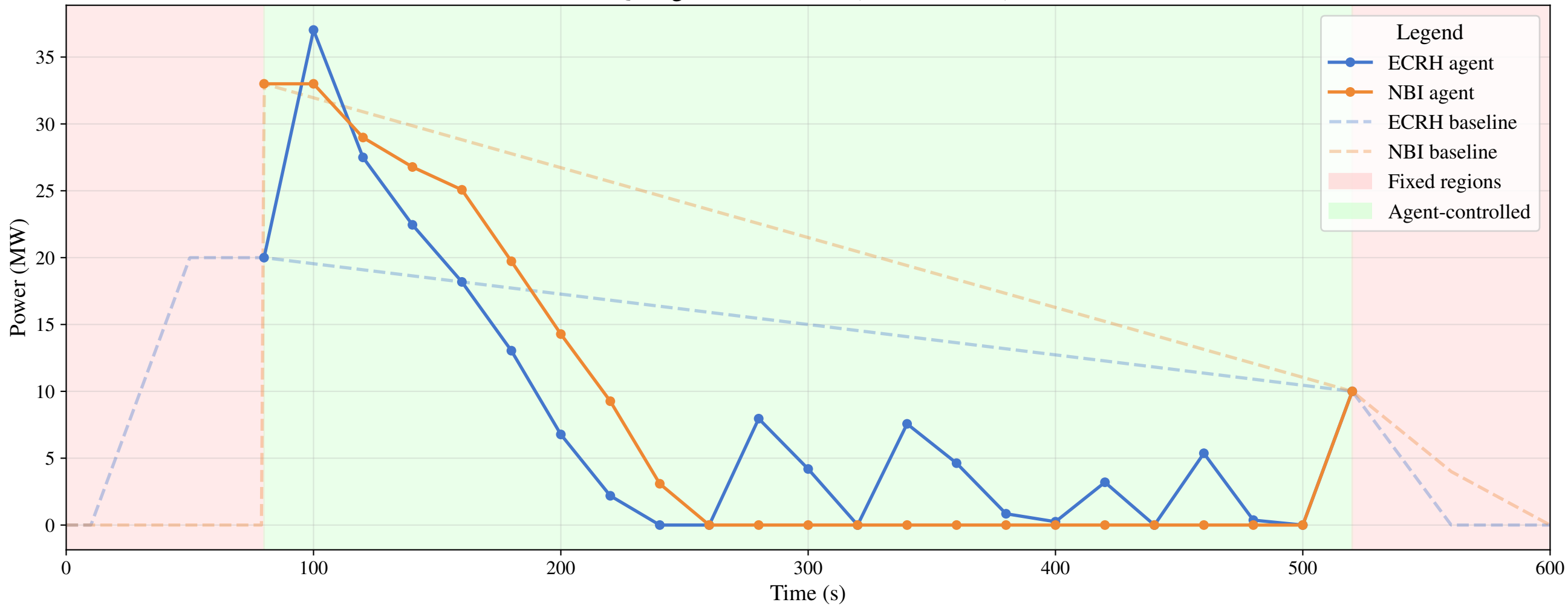
IQL Agent vs. Baseline (reward=51.21)
