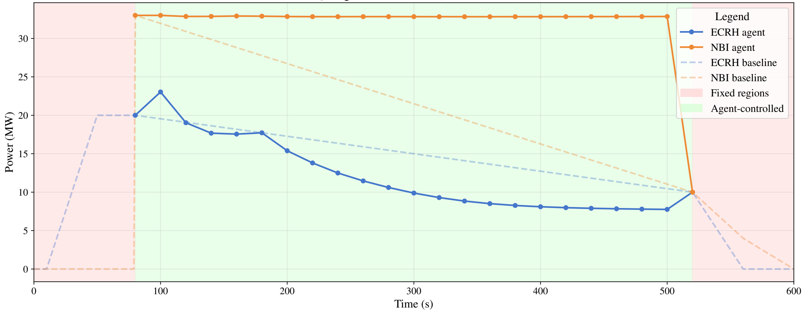
IQL Agent vs. Baseline (reward=11.75)
