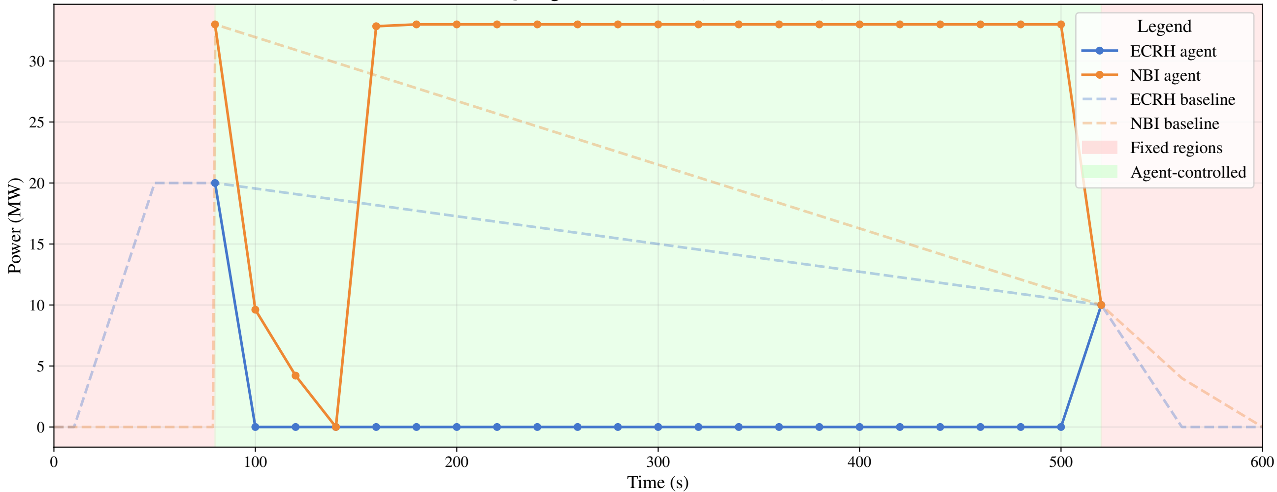
CQL Agent vs. Baseline (reward=26.20)
