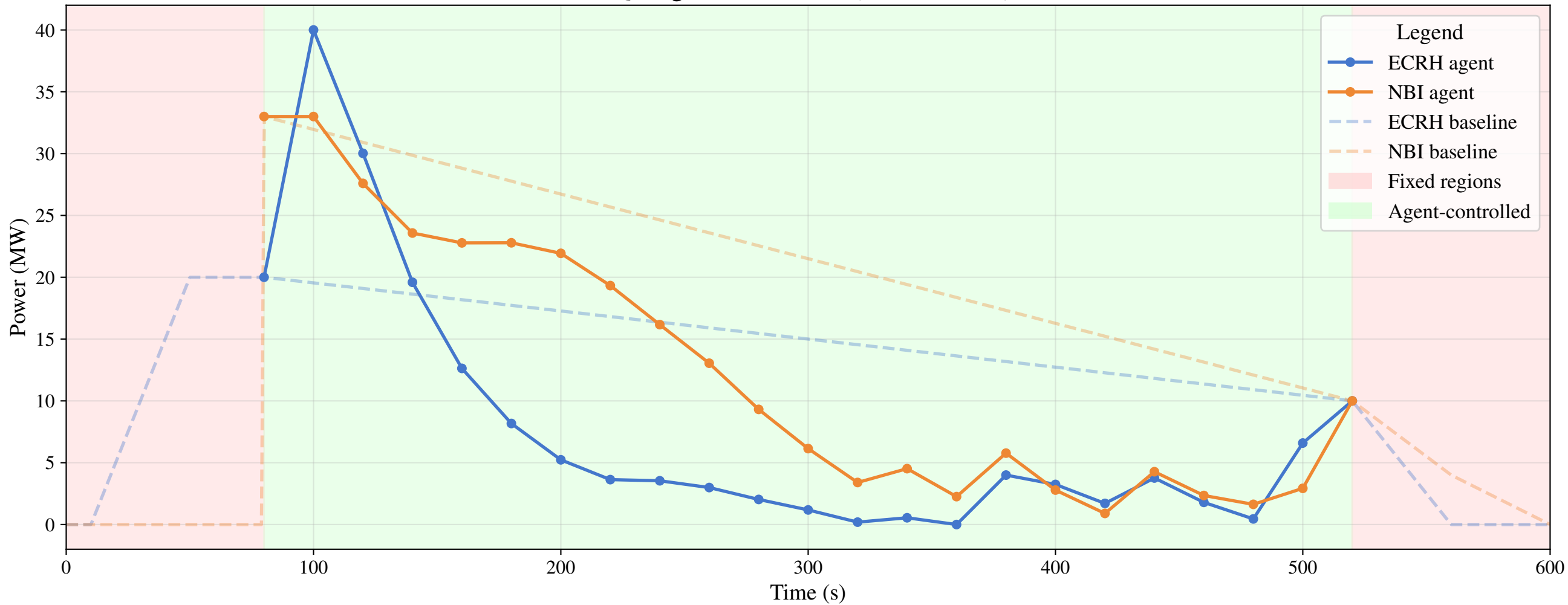
IQL Agent vs. Baseline (reward=43.95)
