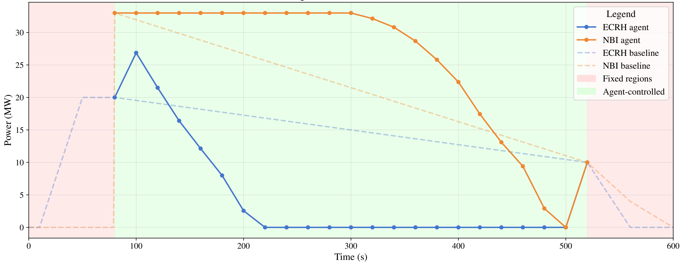
TD3BC Agent vs. Baseline (reward=25.07)
