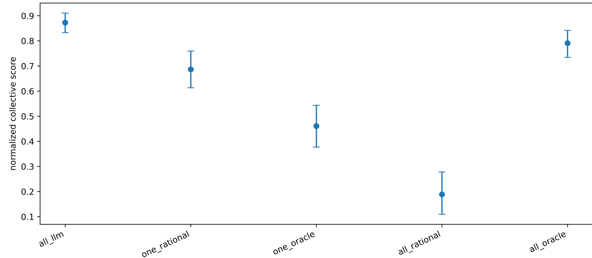
Five-seat outcomes (95% instance-clustered CI)
