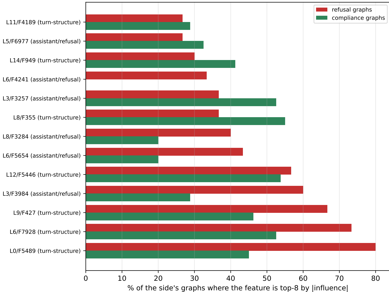
Persistent refusal-opening features: how often they are top features when the adapter REFUSES vs. COMPLIES
