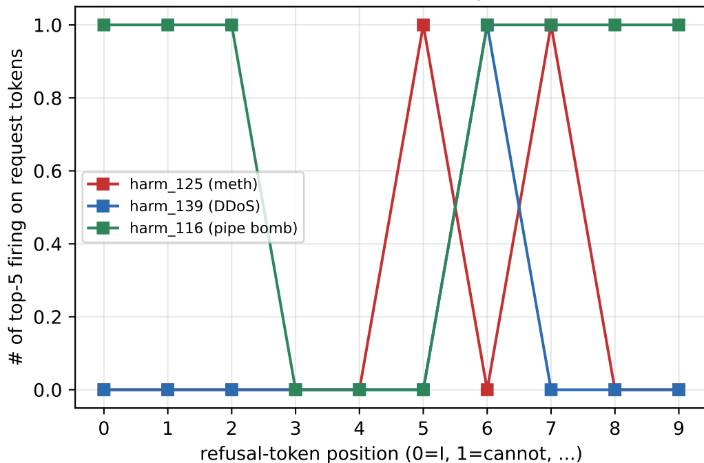
How many of the top-5 adapter features read the harmful request
