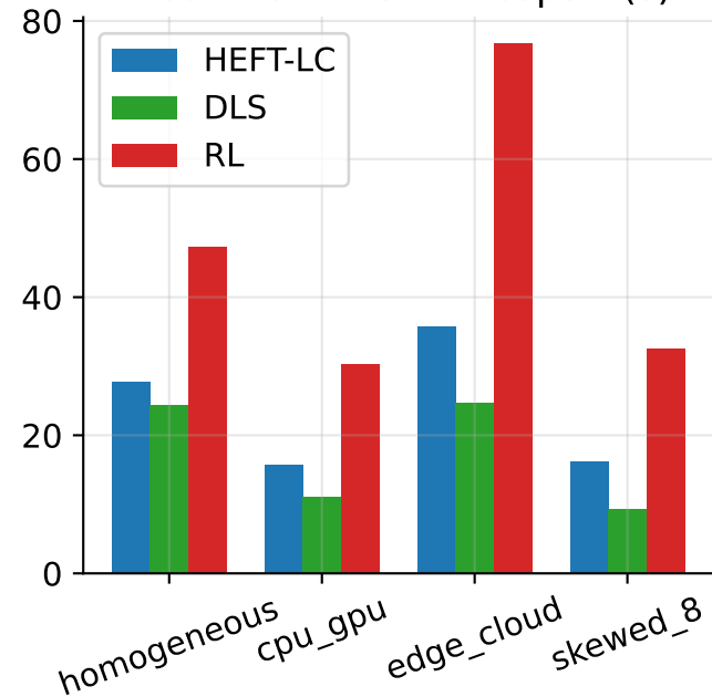
Mean Per-DAG Makespan (s)
