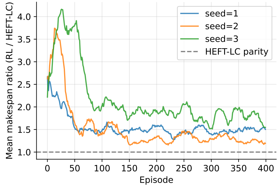
Q-learning convergence
