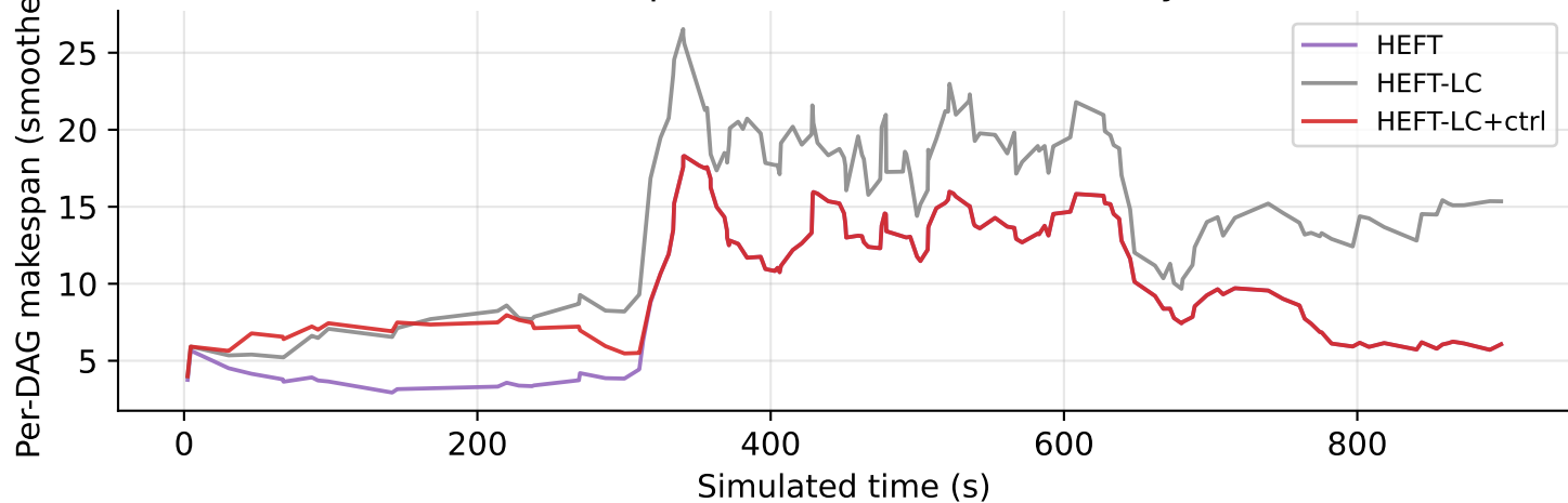
Per-DAG makespan over the non-stationary stream
