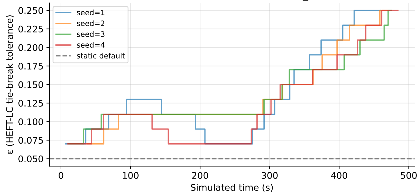
Autonomic adaptation trace (skewed_8 cluster)
