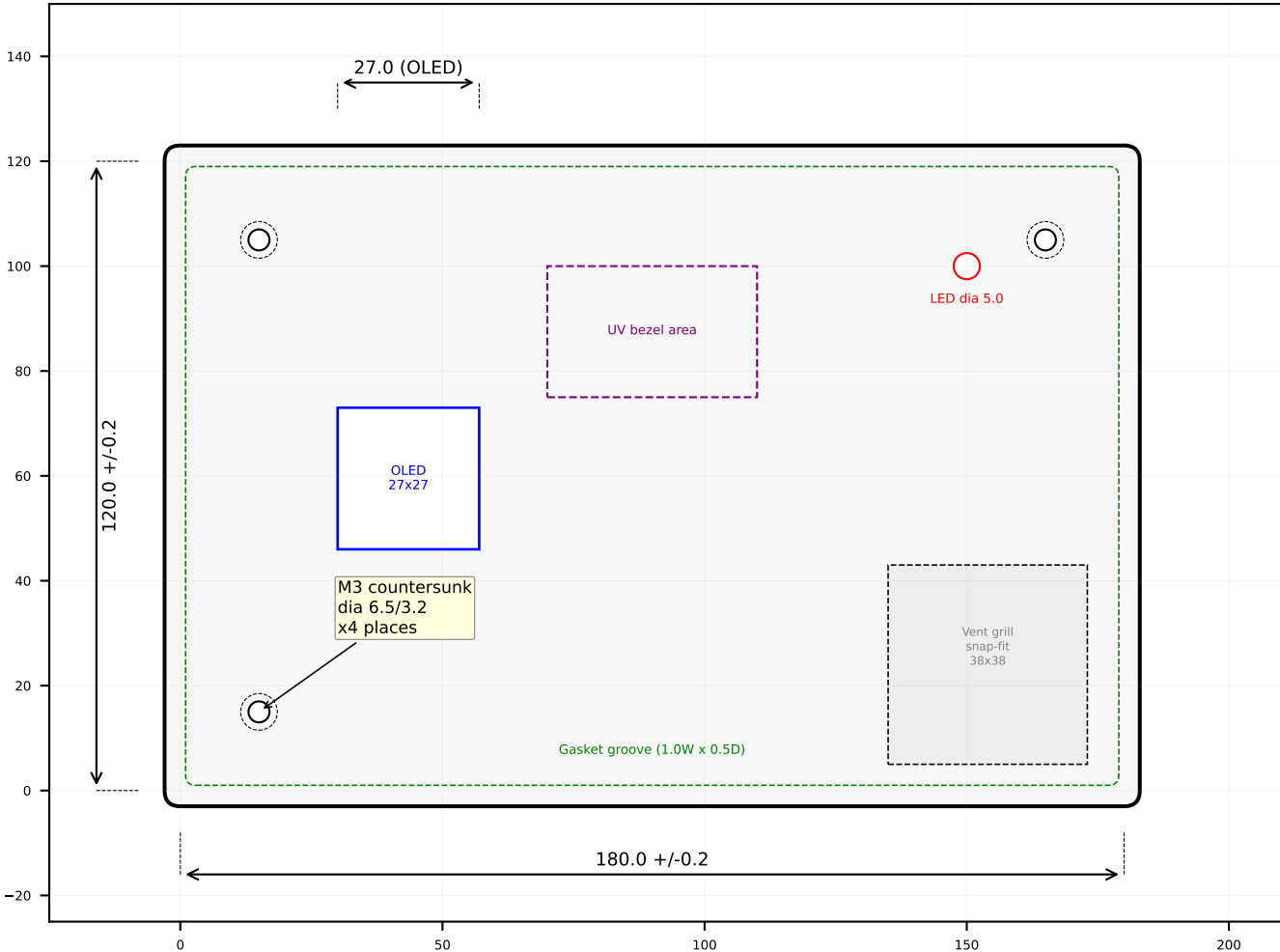
TOP VIEW (exterior)
