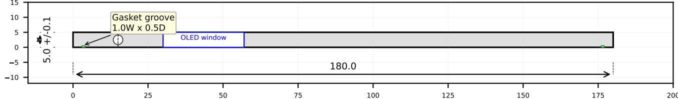
SECTION A-A (cross section)
