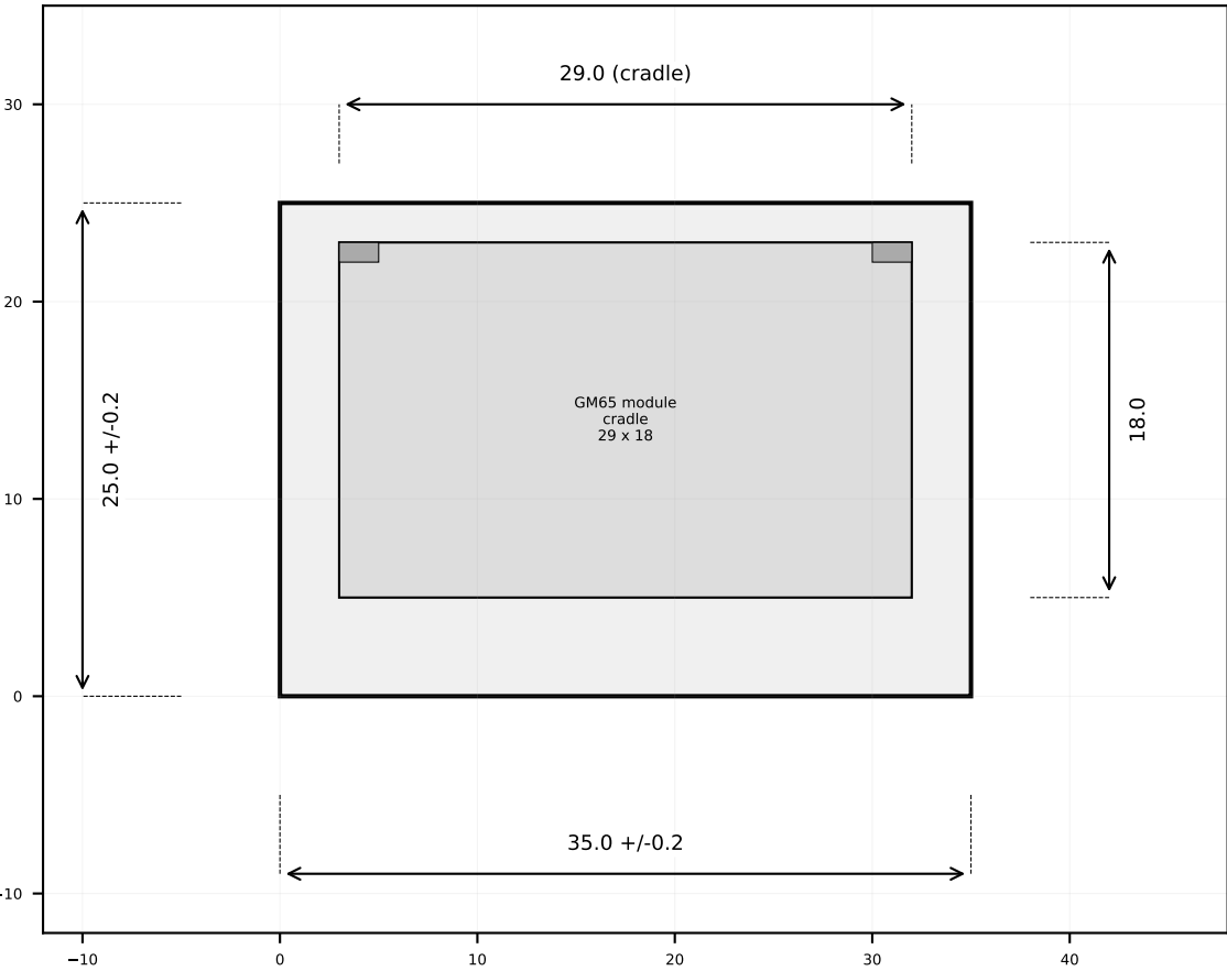
FRONT VIEW
