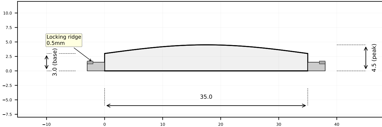
SECTION C-C (profile)
