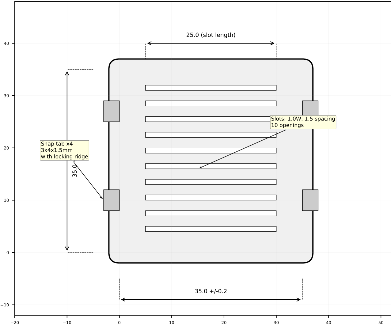
TOP VIEW (exterior face)
