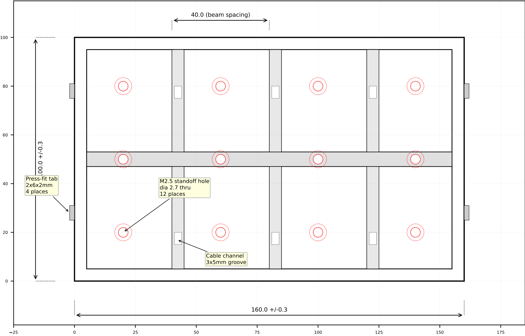
TOP VIEW
