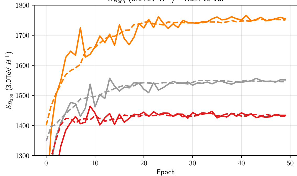
S_{B_{200}} (3.0TeV H^+ ) - Train vs Val
