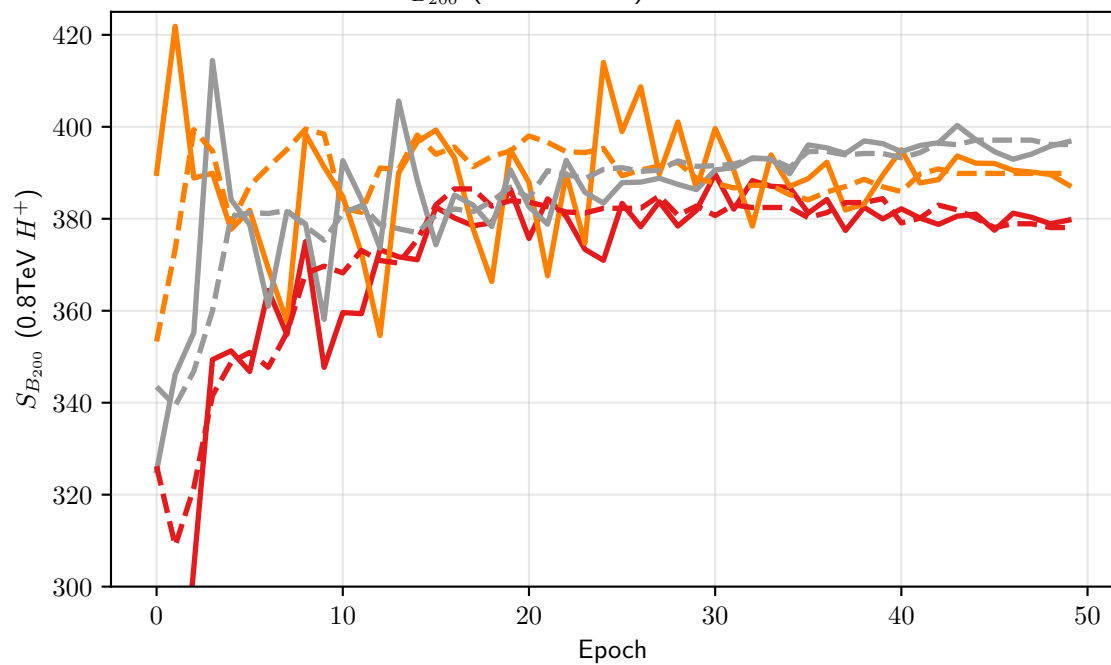
S_{B_{200}} (0.8TeV H^+ ) - Train vs Val
