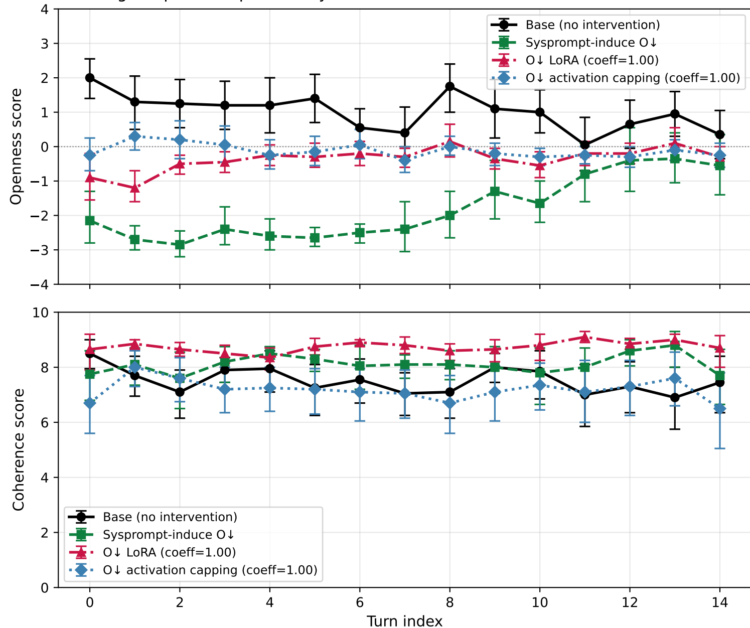
Inducing O↓ persona: per-turn dynamics across induction methods
