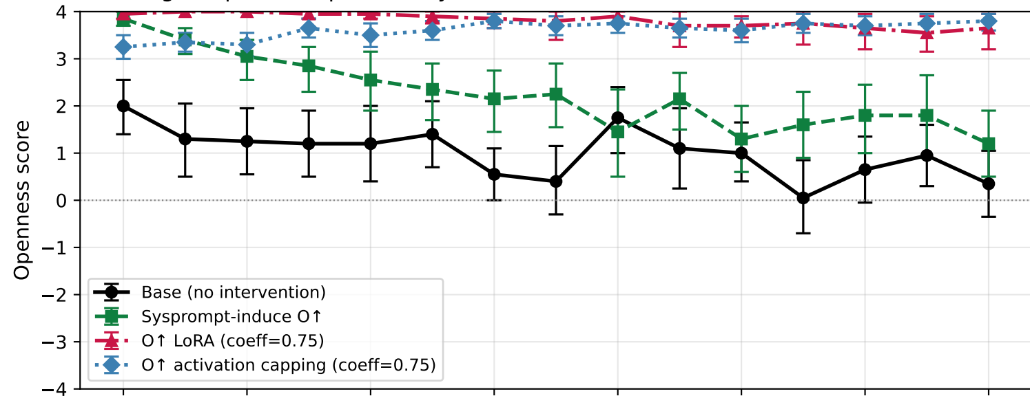
Inducing O \uparrow persona: per-turn dynamics across induction methods
