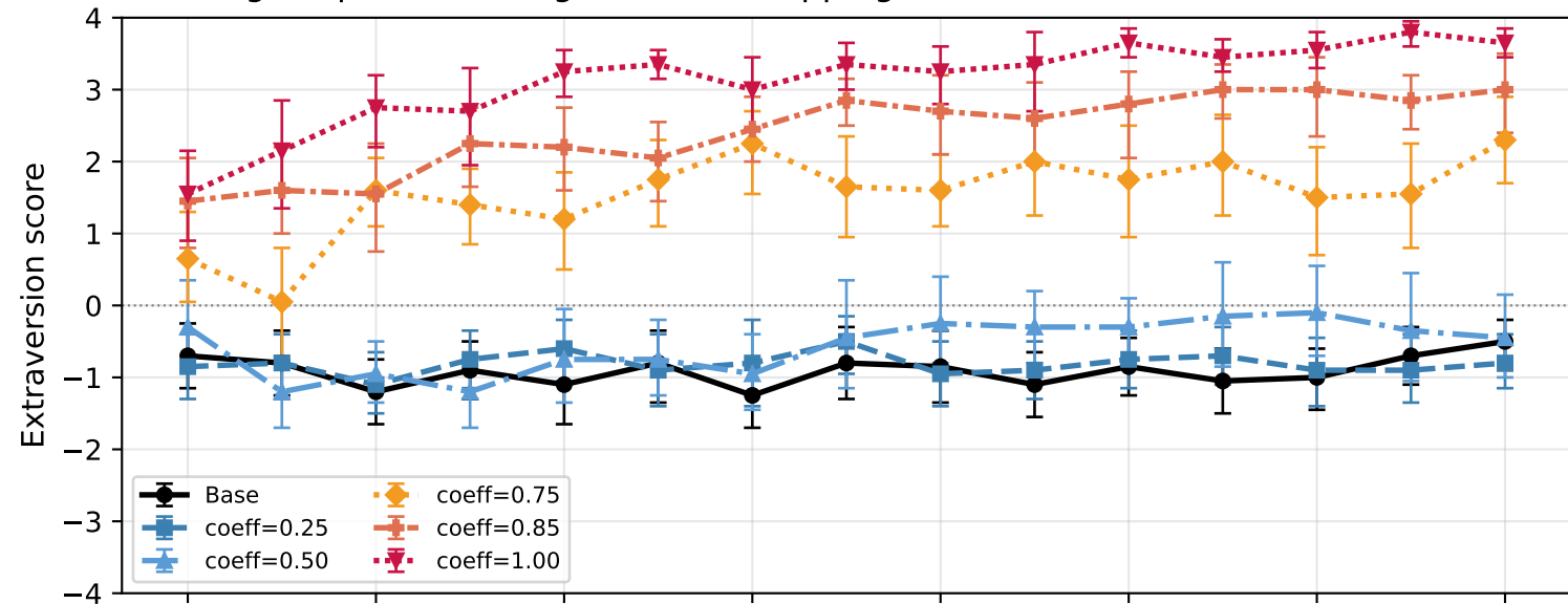
Inducing E \uparrow persona using activation capping at different coefficients
