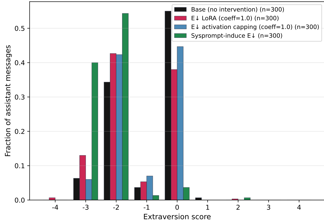
(b) Distribution of per-message scores
