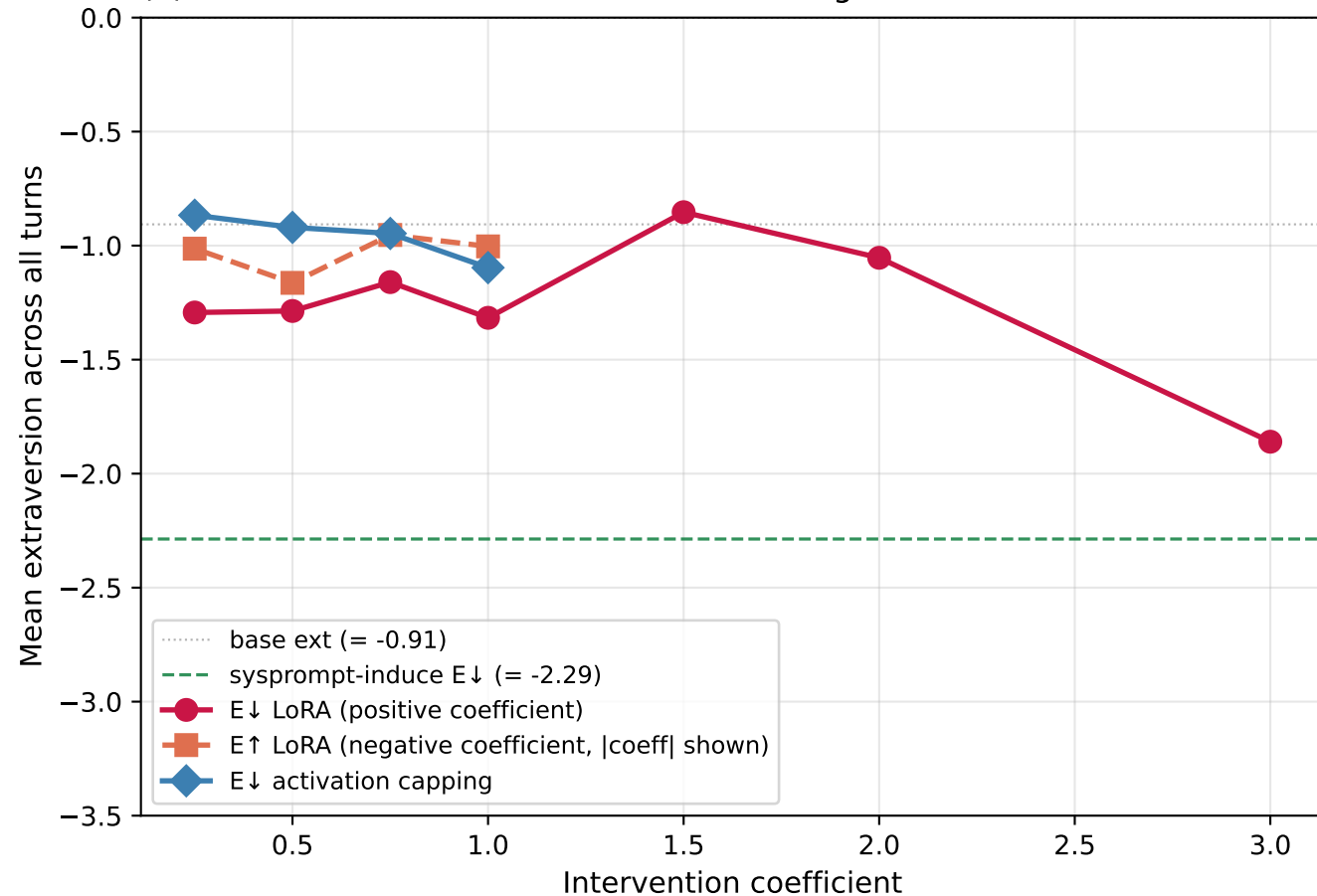
(a) Mean extraversion vs intervention strength
