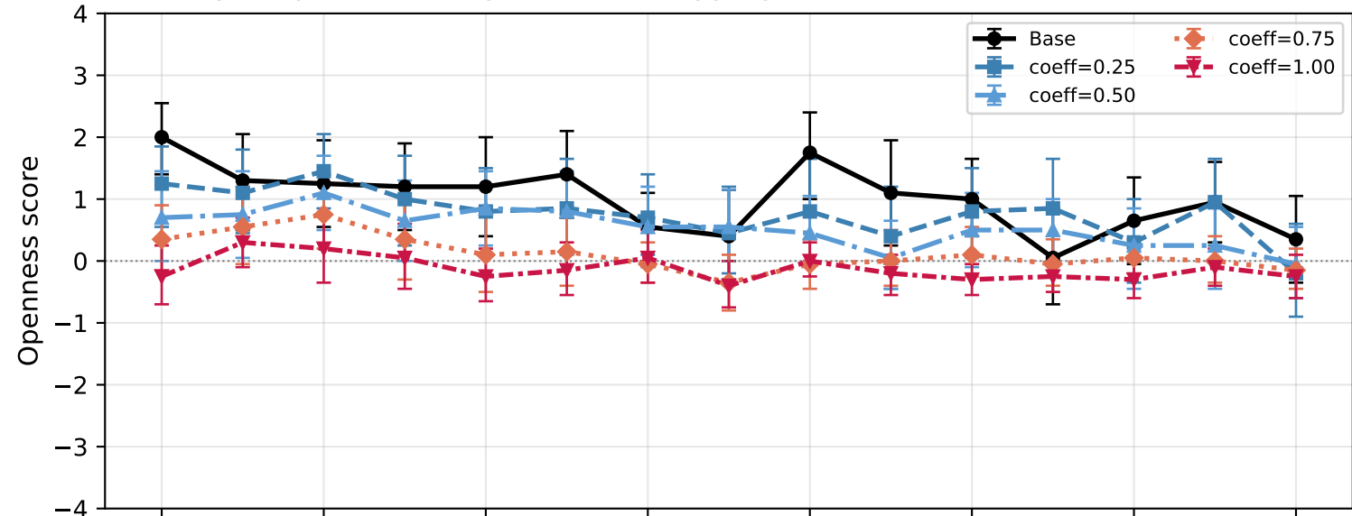
Inducing O↓ persona using activation capping at different coefficients
