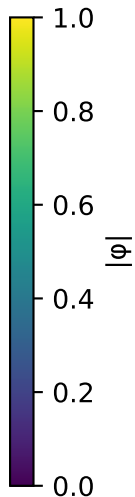
Tucker's |\phi| (combined, n_shared=95)
