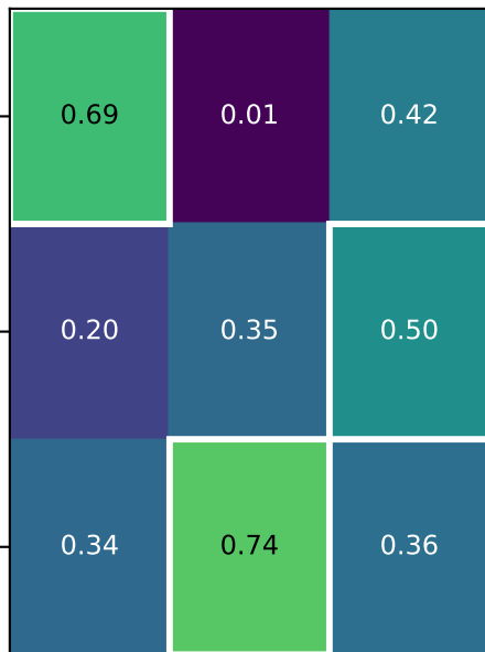
Tucker's |\phi| (combined, n_shared=95)
